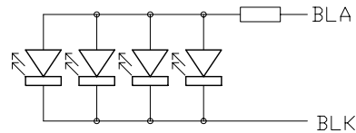
Backlight Circuit (No. of LEDs = 4pcs) Scale=free
